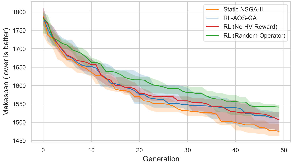
Convergence (Best-So-Far Makespan)
