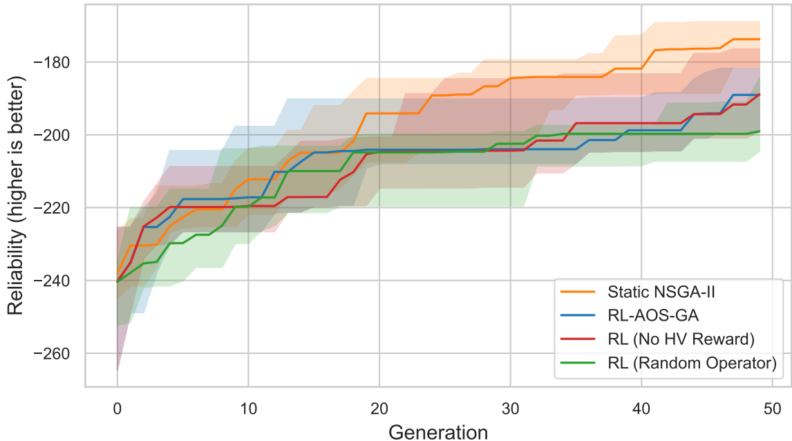
Convergence (Best-So-Far Reliability)
