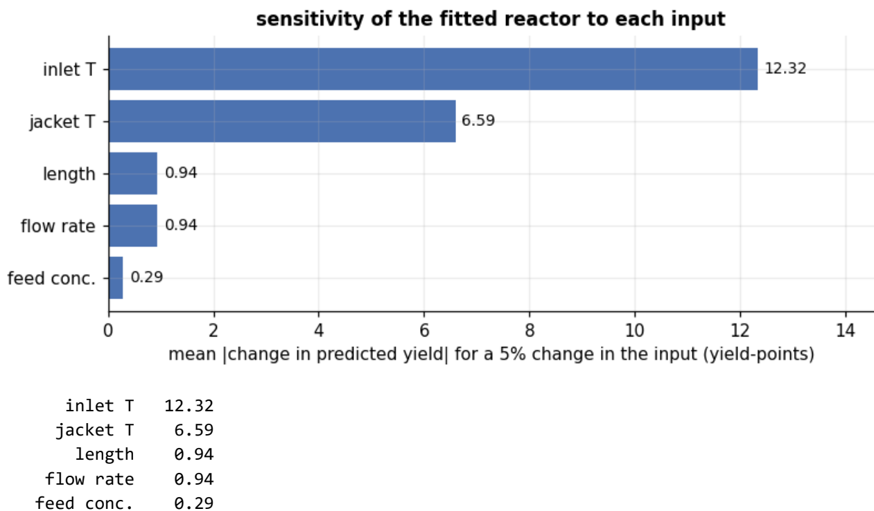
Figure 5. Sensitivity of the fitted model to a 5% change in each input. The two temperatures dominate and feed concentration is last, which is the same conclusion the correlation and the a_1/a_2 cancellation reach by different routes.
