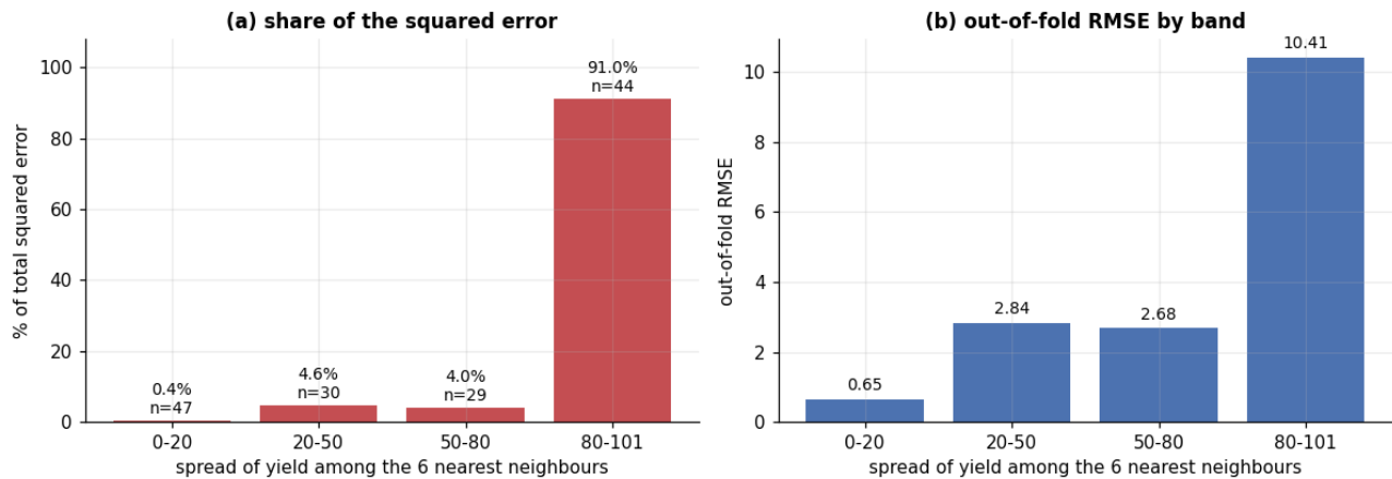
Figure 6. Rows whose local neighbourhood already disagrees carry almost all of the error; the settled majority is predicted almost exactly.
