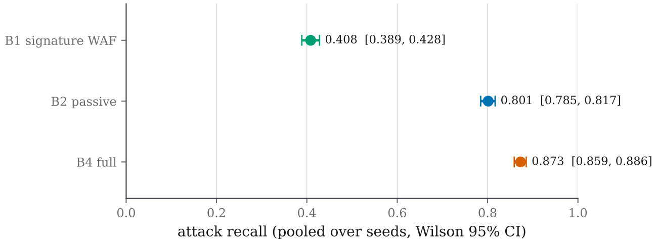
Per-arm recall with 95% confidence intervals (20 seeds)
