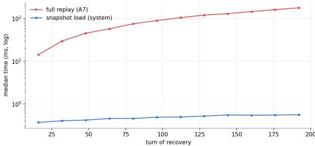
Fig. 12. Median time to rebuild state at each snapshot point (log scale): full replay of the event log (A7) against snapshot loading (the system), over 42 sessions of 200 turns. The plot’s title strip, which lists the consistency rates of Table XIV, is cropped.
