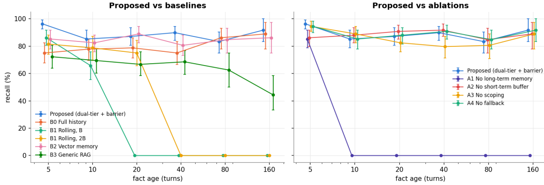
Fig. 5. Recall by fact age on held-out worlds with 95% bootstrap intervals. Left: F4 against the baselines; the rolling contexts fall to zero once a fact leaves the window (B1 after age 10, B1 \times 2 after age 20), while F4 and B2 stay flat and generic RAG (B3) declines to 44.4% at age 160. Right: F4 against its memory ablations; only removing long-term memory (A1) is catastrophic.
