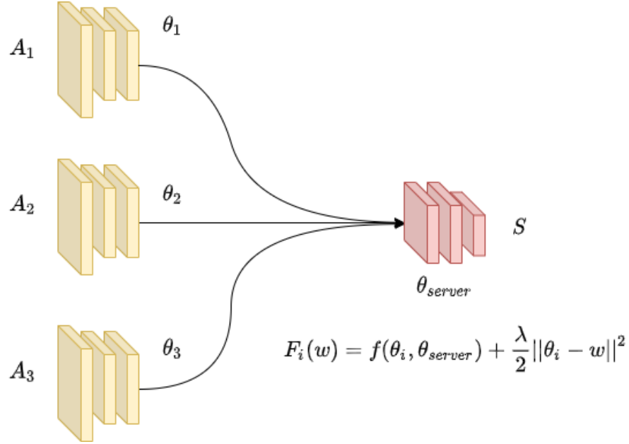
Figure 1. The proposed approach for personalized and privacy aware deep learning. A_1 , A_2 , and A_3 are clients, S is the server, \theta_i are the weights for the corresponding client, \theta_{server} are the weights for the server, w are weights of a reference global model, and F_i(w) is the loss function of the i th client.
