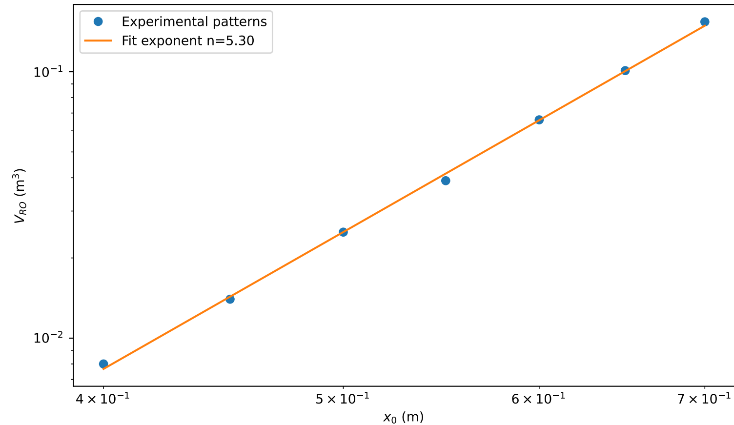
Region-of-origin scaling relation
