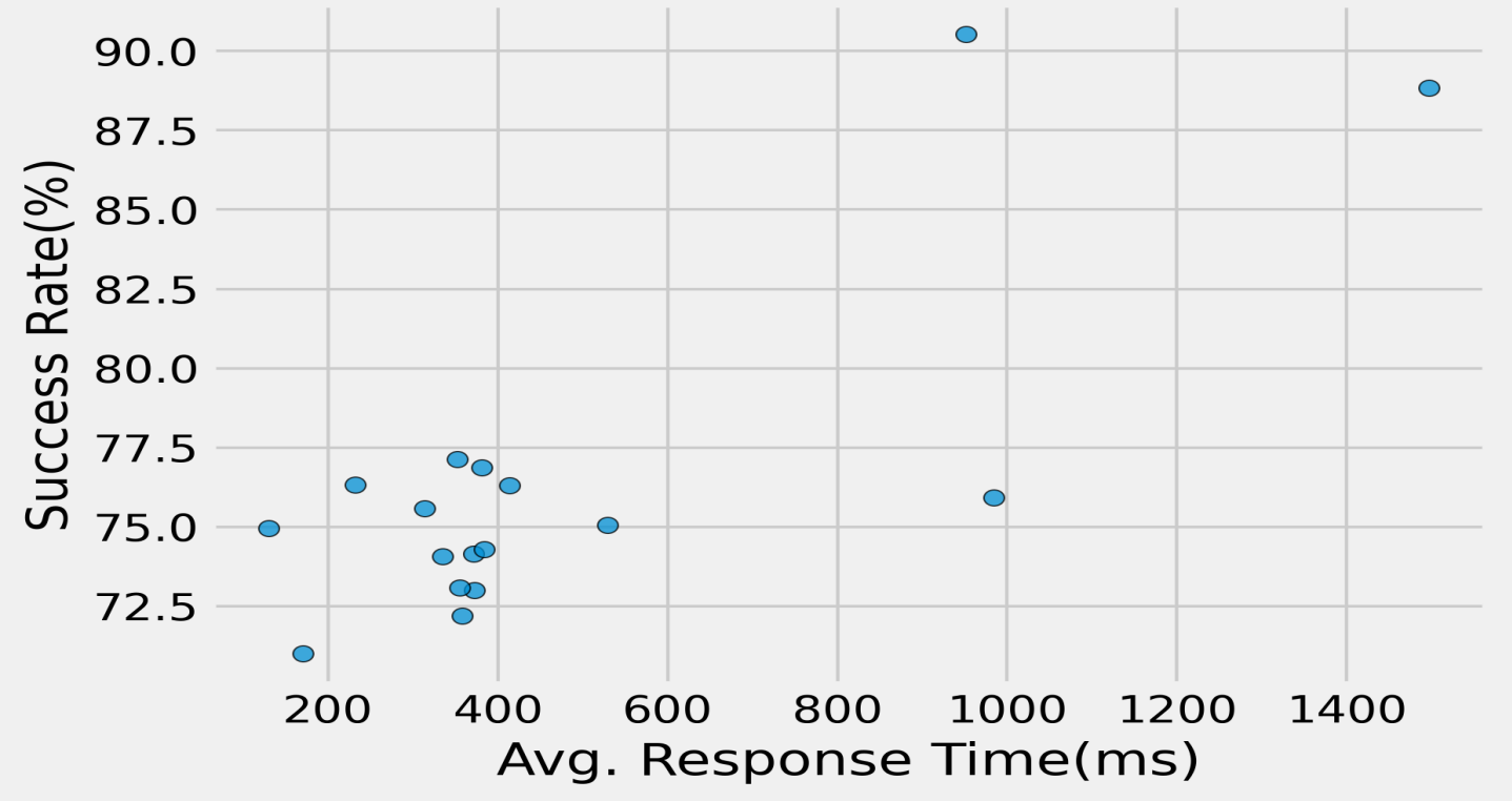
Avg Response Time V/S Success Rate
