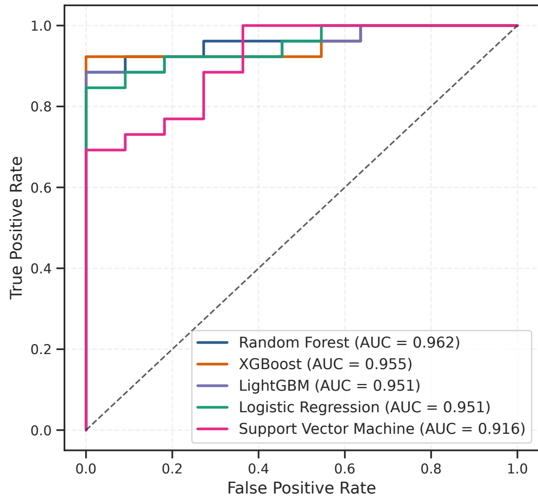
ROC Curves (Experiment 2: Without CNA Burden)
