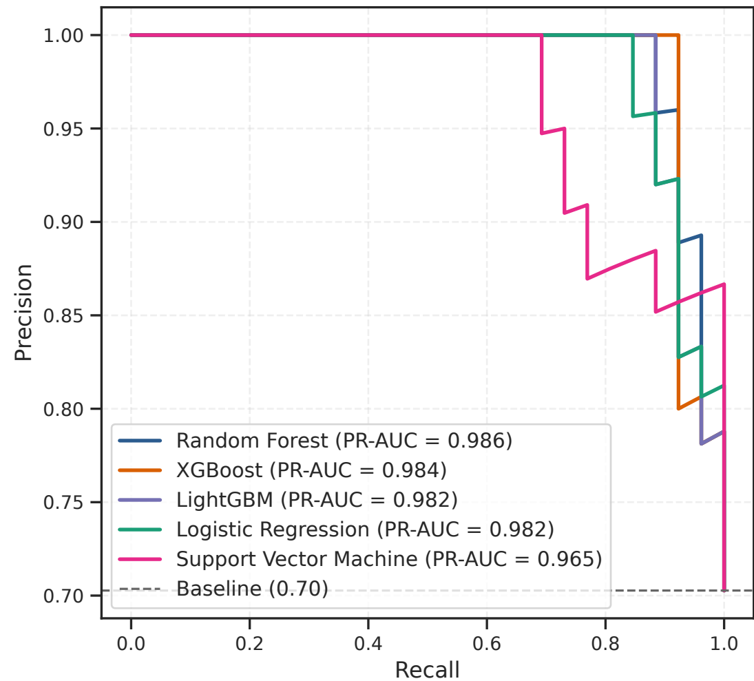
PR Curves (Experiment 2: Without CNA Burden)
