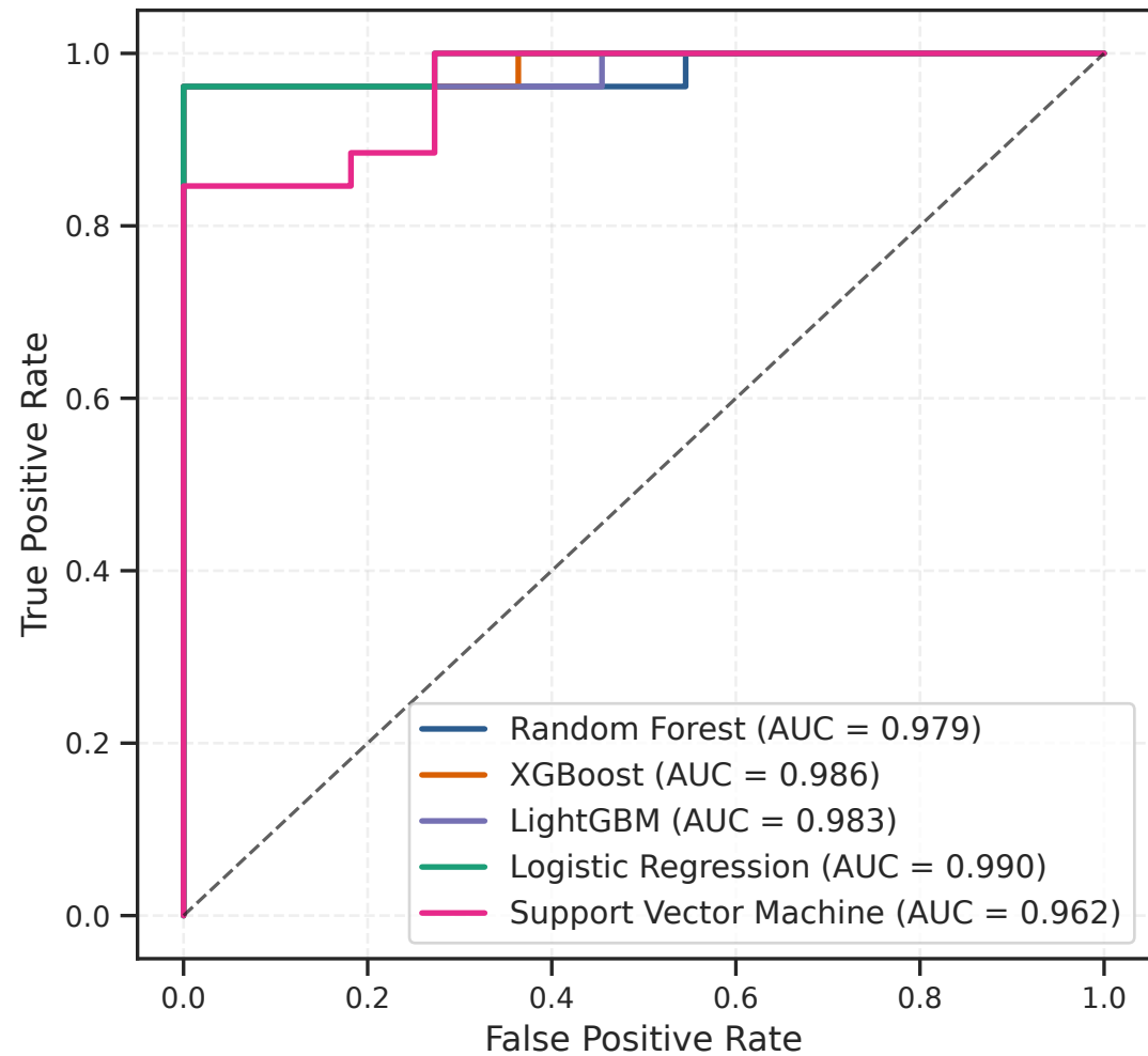
ROC Curves (Experiment 1: With CNA Burden)
