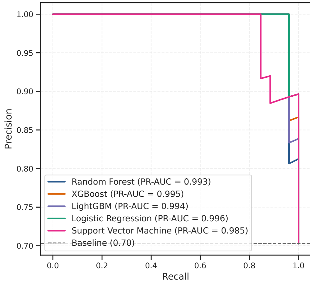
PR Curves (Experiment 1: With CNA Burden)
