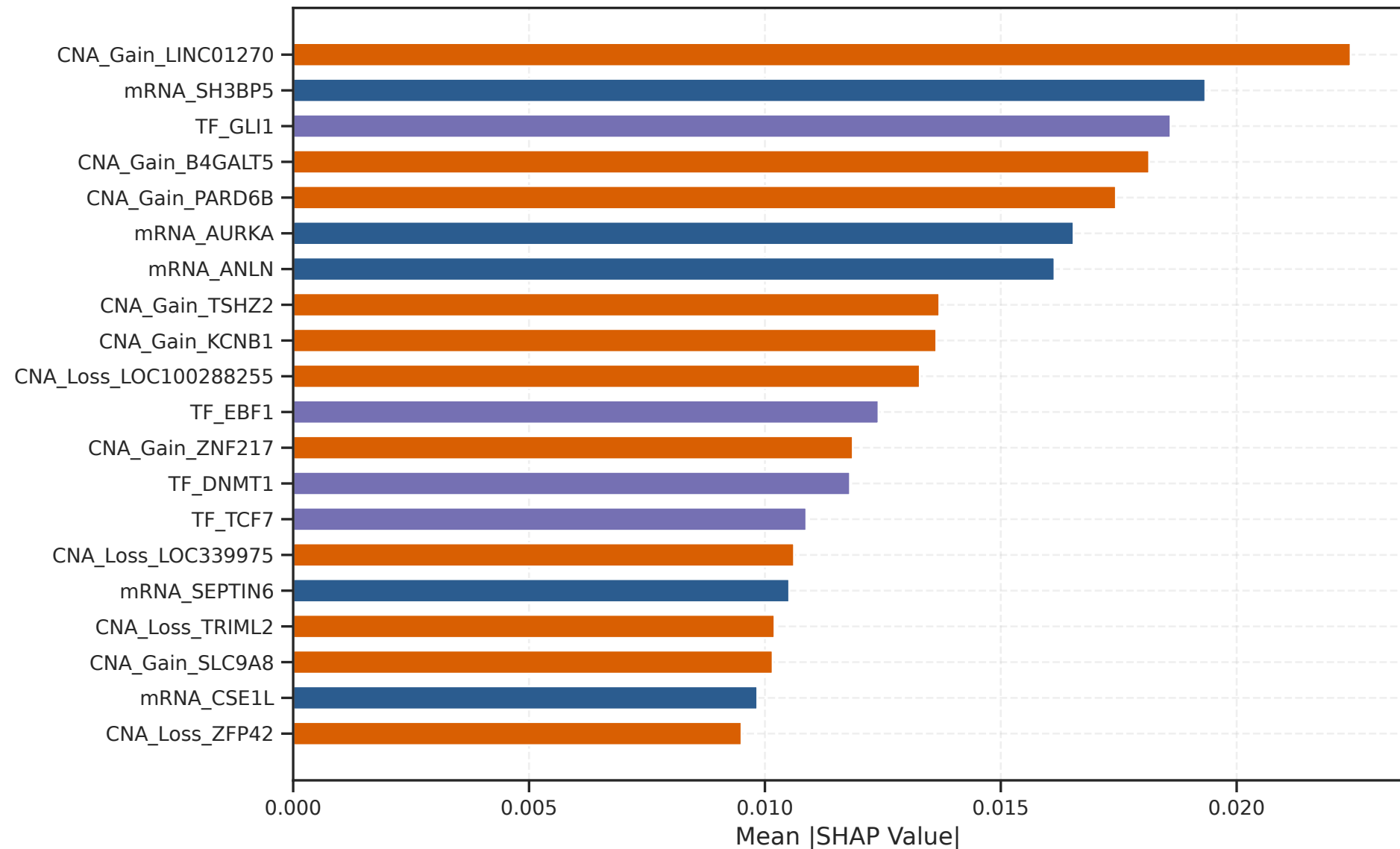
Top 20 Multi-Omics Biomarkers (Experiment 2: Without CNA Burden)
