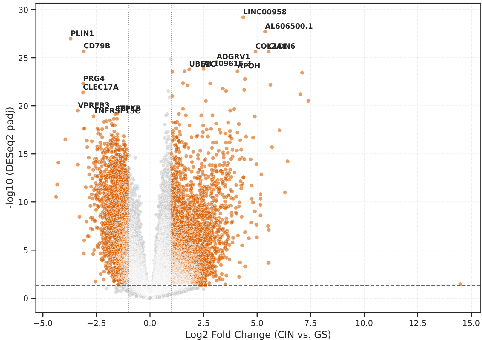
DESeq2 Differential Expression Volcano Plot: CIN vs. GS Subtypes
