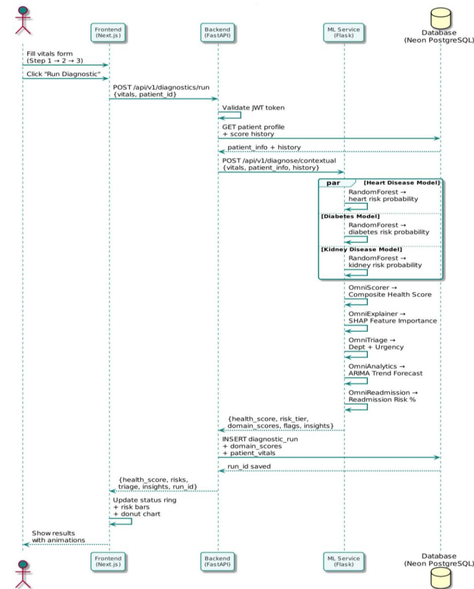
Fig 5.5 : Sequence Diagram – AI Diagnostic Run Flow
