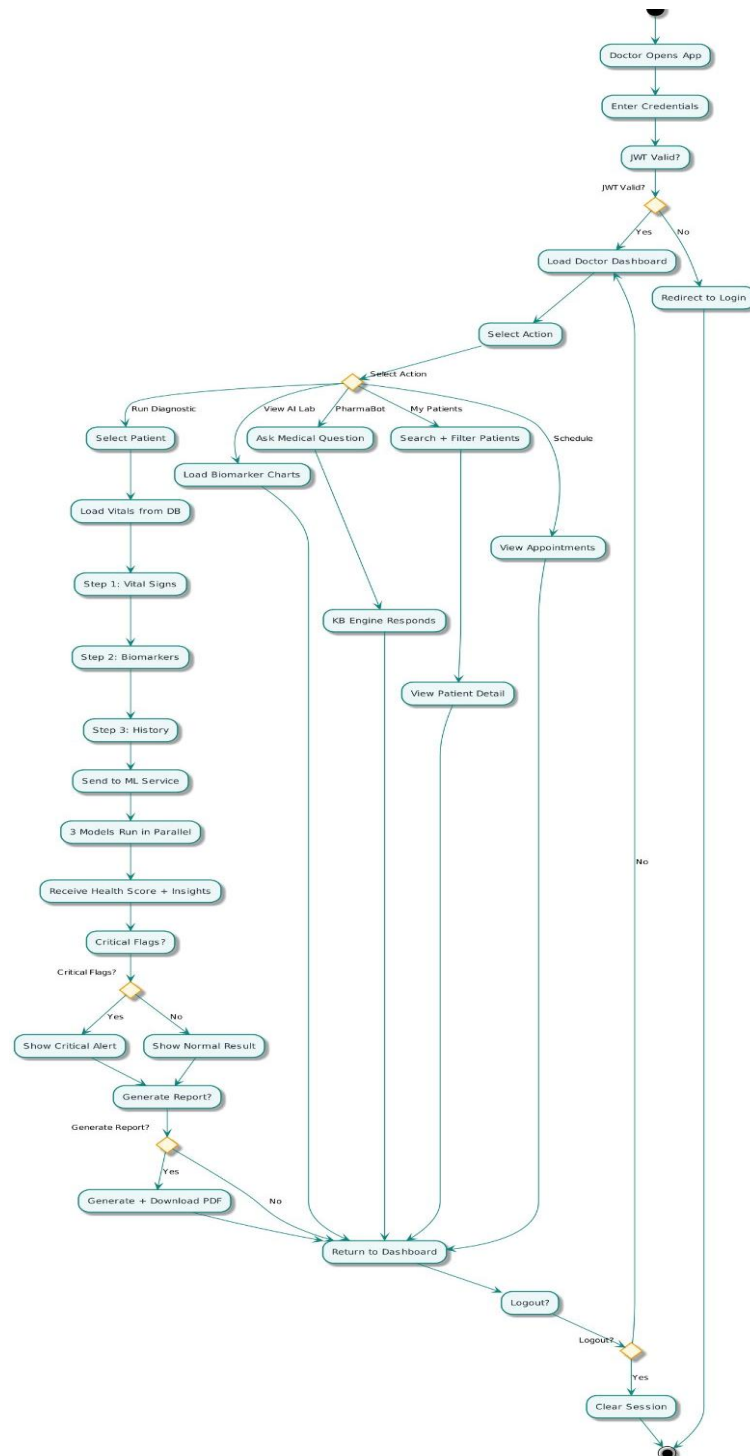
Fig 5.3 : Activity Diagram – Doctor Workflow
