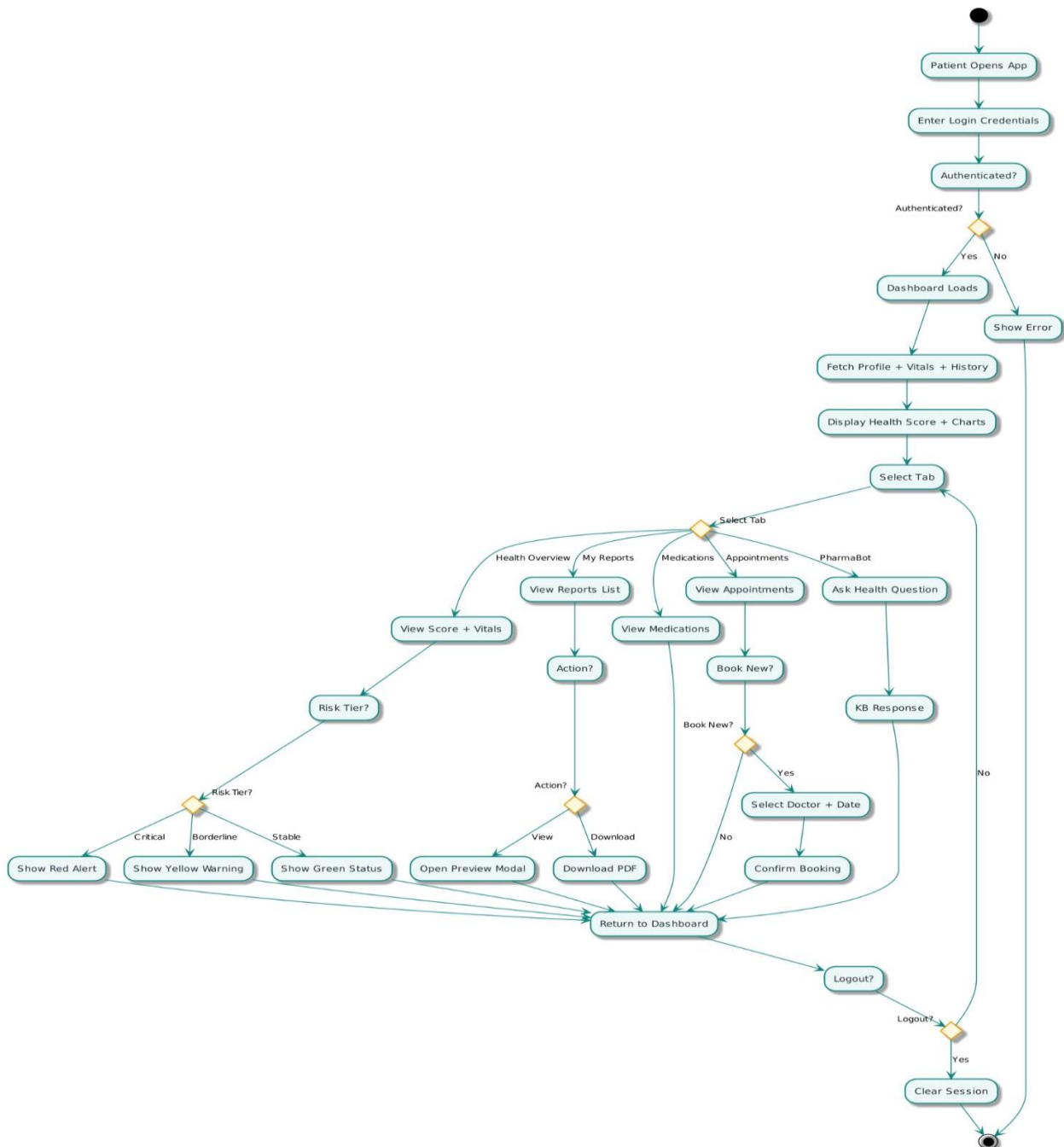
Fig 5.4 : Activity Diagram – Patient Journey
