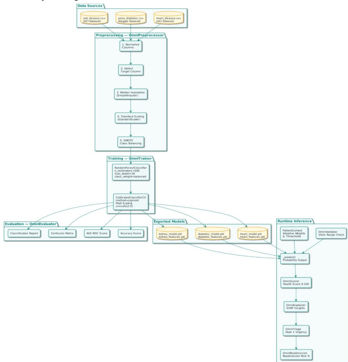
Fig 5.10 : ML Pipeline Diagram – Training and Inference
