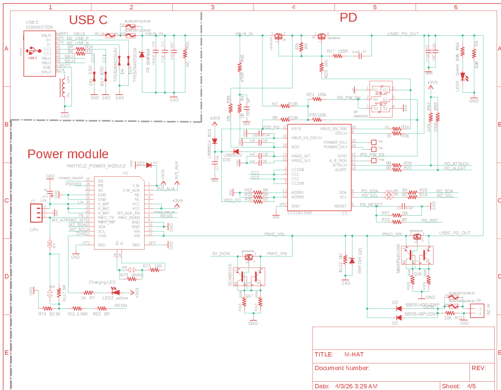
SCHEMATICS PAGE 4
