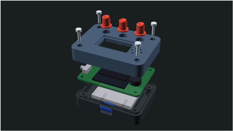
Figure 4: Exploded Multi-Tier Hardware Assembly (1920 × 1080 High-Resolution Projection) Tier 1: Base Shell • Tier 2: LiPo Battery & TP4056 • Tier 3: Main PCB • Tier 4: Lid Bezel • Tier 5: 3x Buttons • Tier 6: M2 Fasteners
