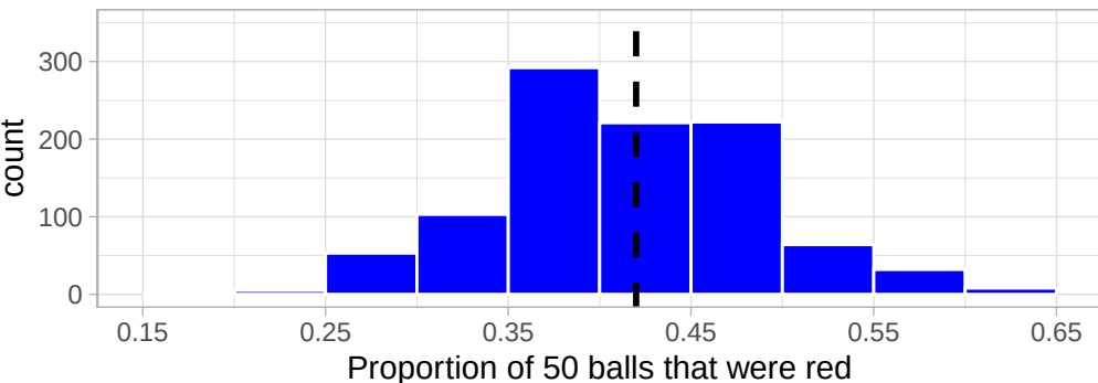
Bootstrap distribution: similar shape and spread but different c
