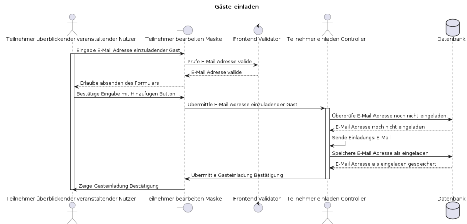
Figure 2: F004_gaesteEinladen_seq.png
