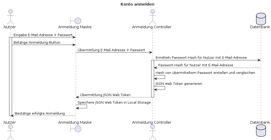
Figure 2: F011_kontoAnmelden_seq.png
