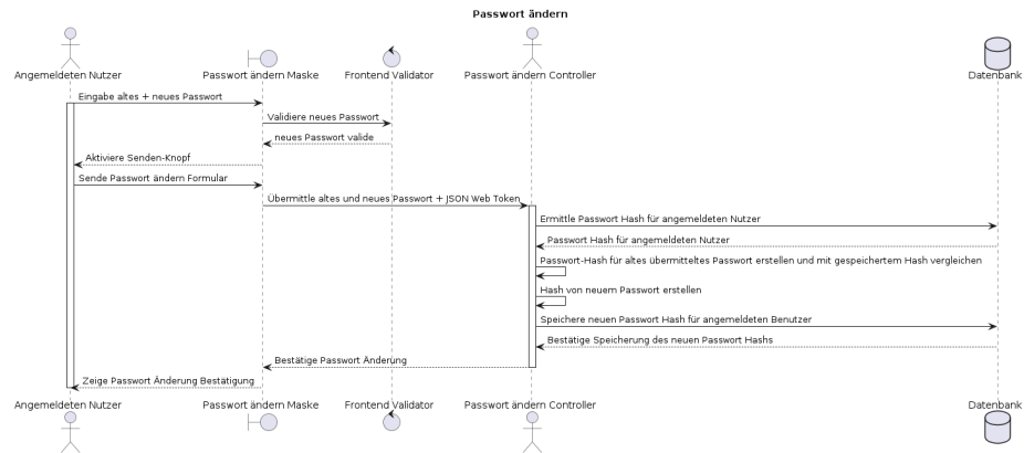
Figure 2: F013_passwortAendern_seq.png
