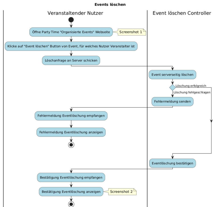
Figure 1: F003_eventsLoeschen_act.png
