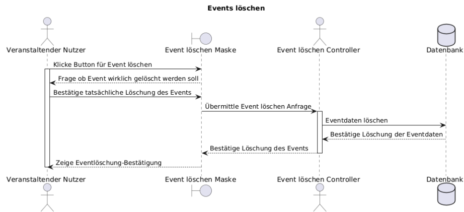
Figure 2: F003_eventsLoeschen_seq.png
