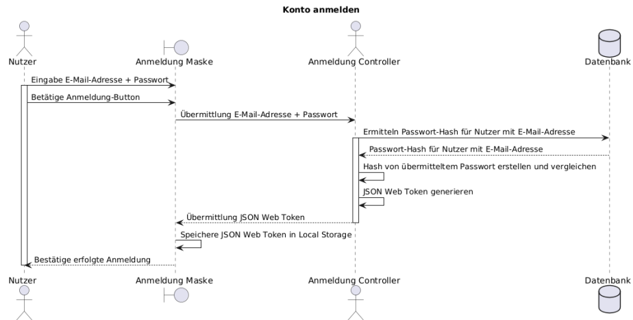
Figure 2: F011_kontoAnmelden_seq.png
