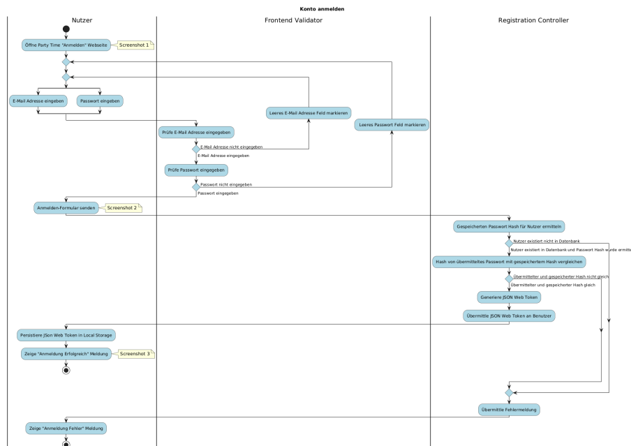
Figure 1: F011_kontoAnmelden_act.png
