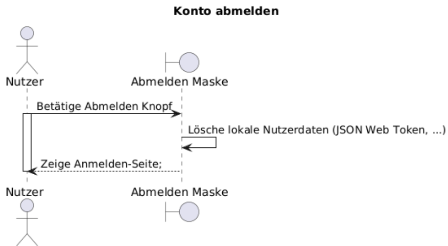
Figure 2: F012_kontoAbmelden_seq.png
