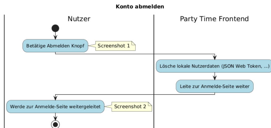
Figure 1: F012_kontoAbmelden_act.png
