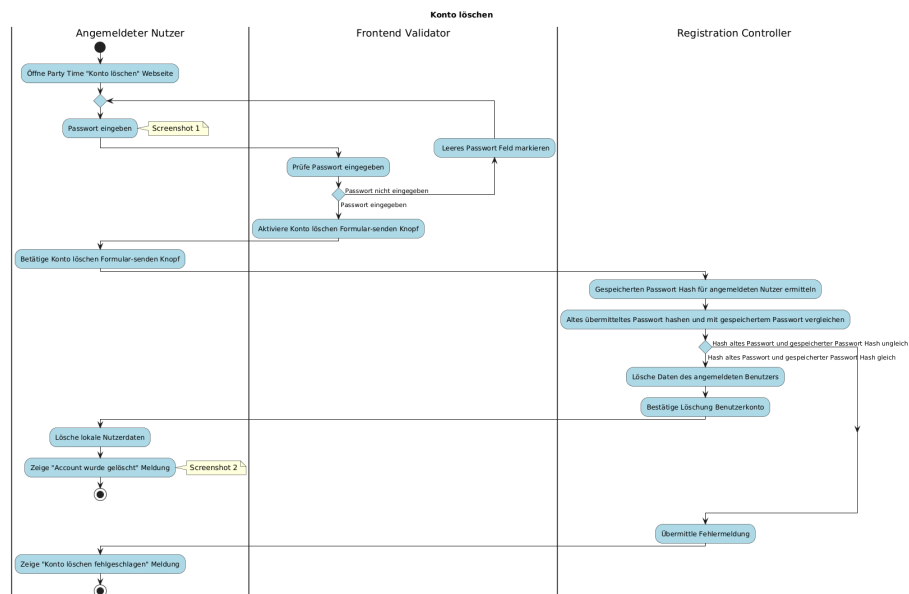
Figure 1: F015_kontoLoeschen_act.png
