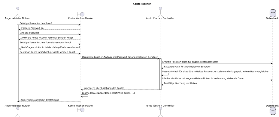
Figure 2: F015_kontoLoeschen_seq.png
