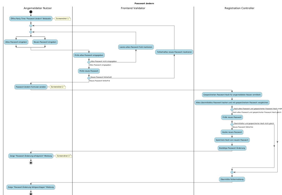
Figure 1: F013_passwortAendern_act.png
