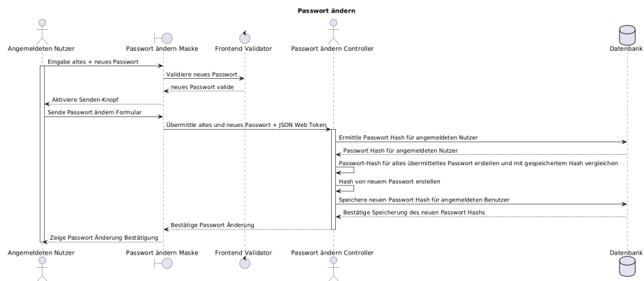
Figure 2: F013_passwortAendern_seq.png
