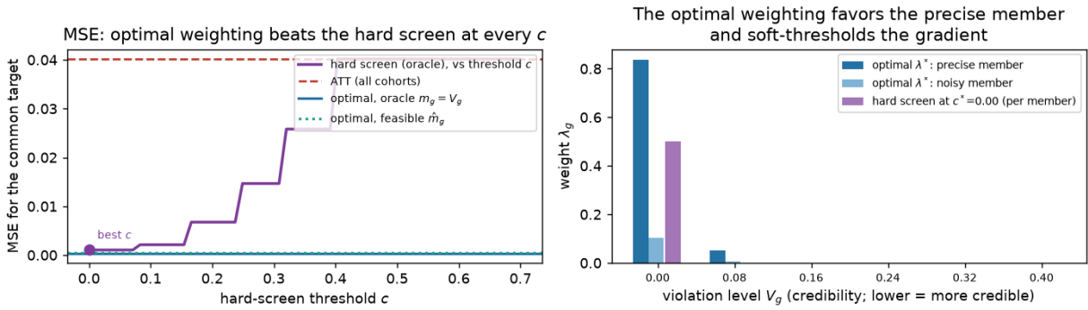
Figure 3: Optimal credible weighting (Proposition 11) versus the hard flatness screen, homogeneous effects so every procedure targets the same value. Left: MSE against the hard-screen threshold c ; the optimal weighting, oracle and feasible, lies below the hard-screen curve at every c and below the ATT. Right: weights at each violation level; the optimal weighting loads on the precise member of each pair and soft-thresholds the credibility gradient, where the hard screen weights retained cohorts equally.
