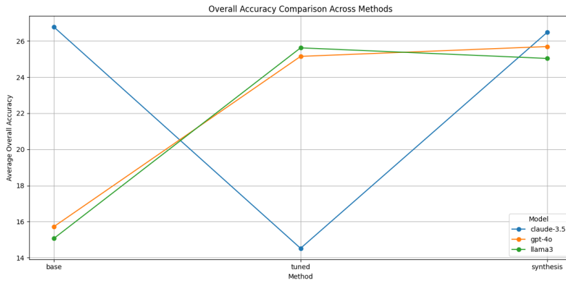
Fig. 11: Average overall accuracy per model and method (manual JSON).
