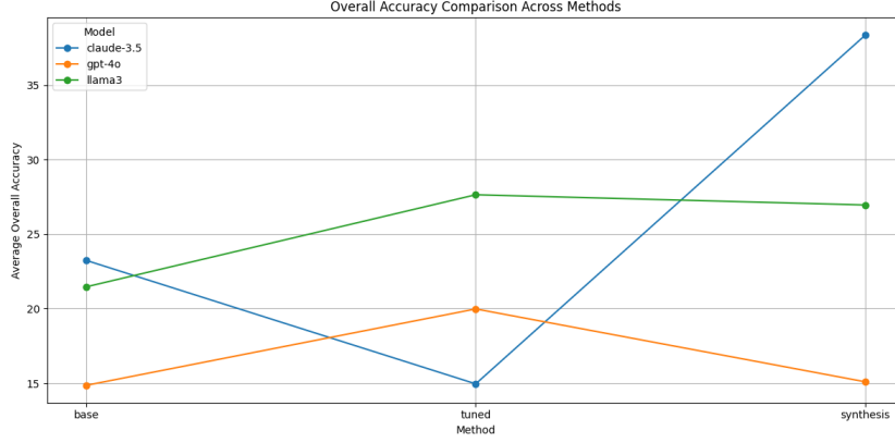
Fig. 13: Average overall accuracy per model and method (LLM-extracted JSON).
