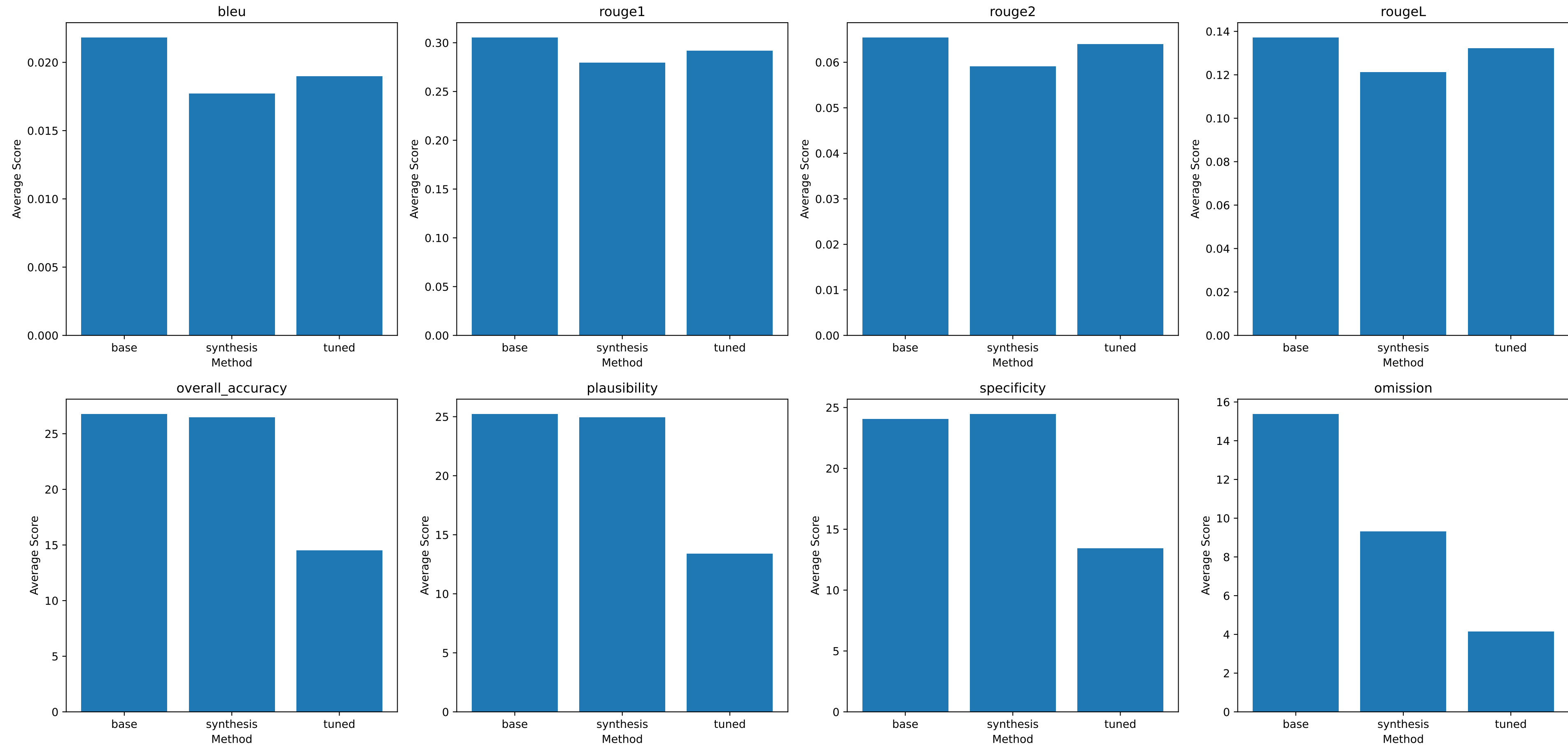
Claude Evaluation (Data Prepared Manually)
