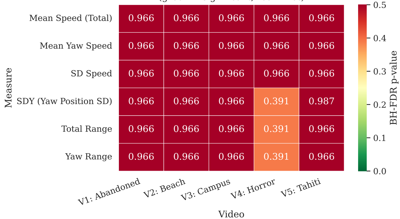
All Measures: BH-FDR Corrected p-Values (green = significant, red = not)
