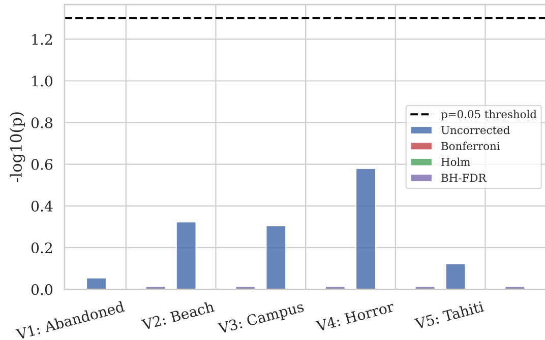
Mean Speed: p-Values Under Different Correction Methods
