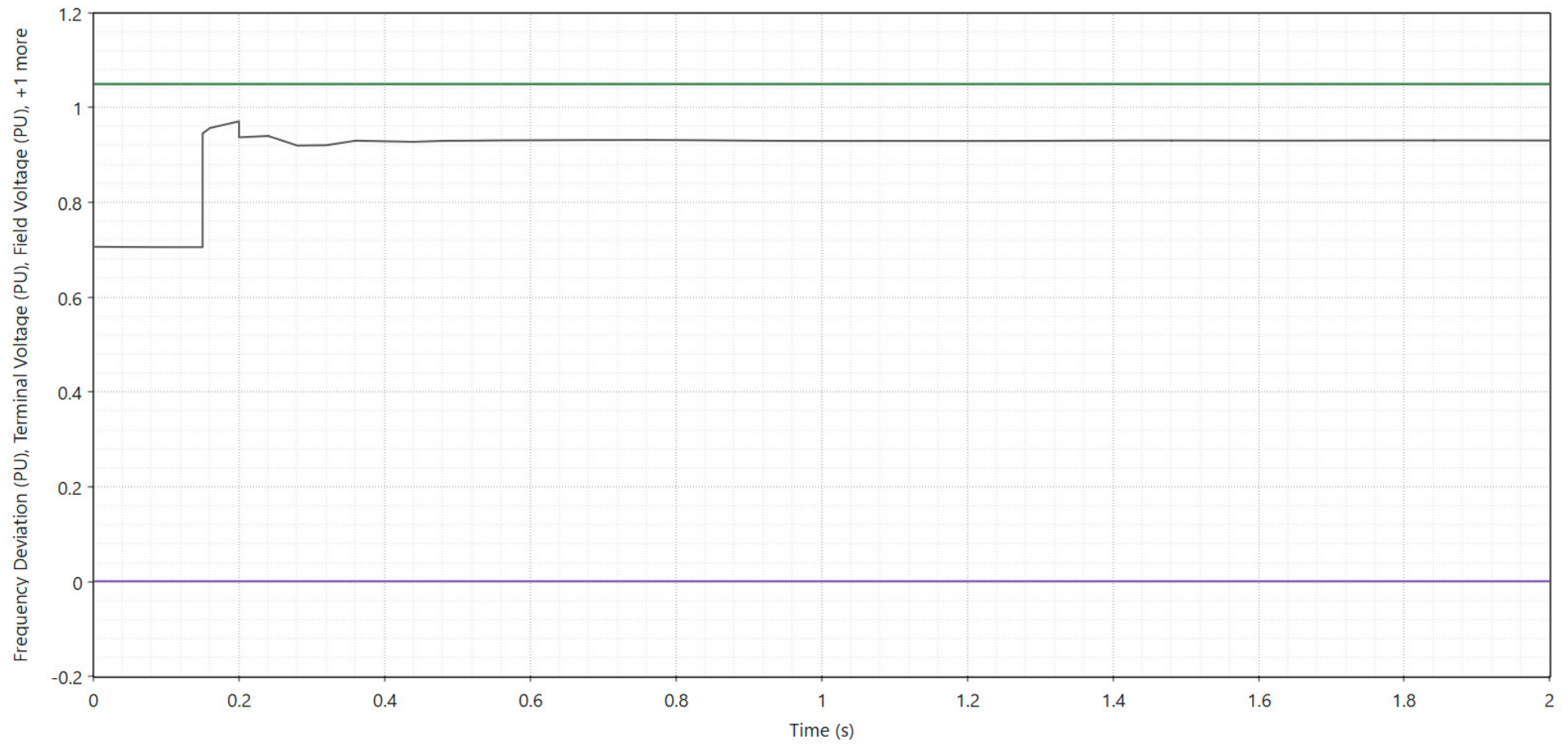
Synchronous machines [1] - Frequency Deviation (PU), Terminal Voltage (PU), Field Voltage (PU), +1 more
