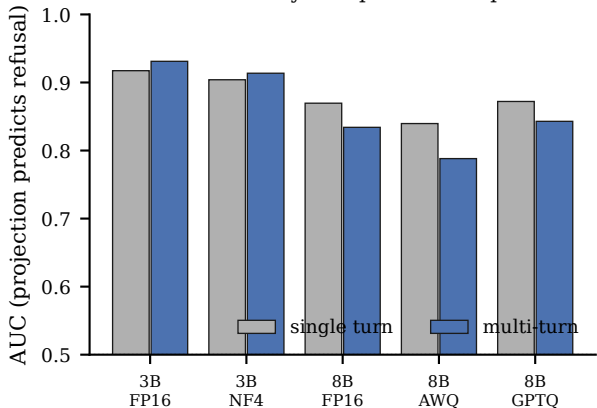
Refusal direction stays coupled under quantization
