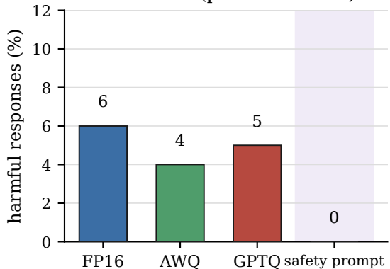
(b) Harm is flat too; a safety prompt cuts it to 0 (positive control)
