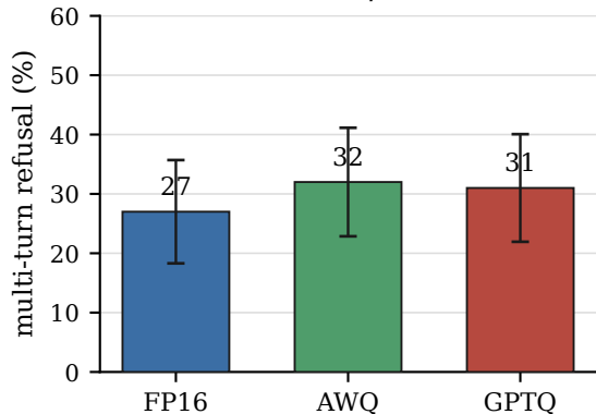
(a) Refusal is flat across precision (Cochran Q p = 0.12 )
