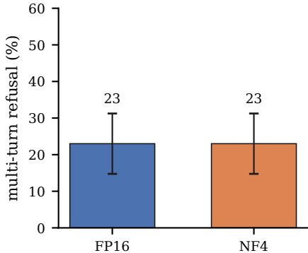
Multi-turn (CoSafe) refusal by precision Llama-3.2-3B Llama-3.1-8B
