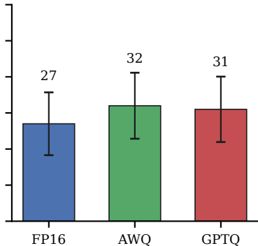
Multi-turn (CoSafe) refusal by precision Llama-3.2-3B Llama-3.1-8B
