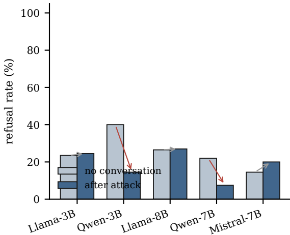
CoSafe
