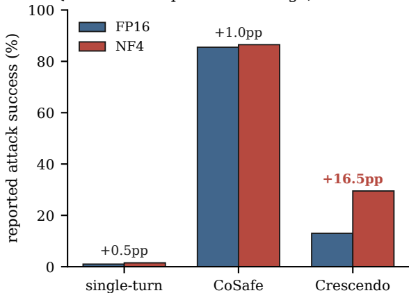
Qwen-3B: one precision change, three attacks
