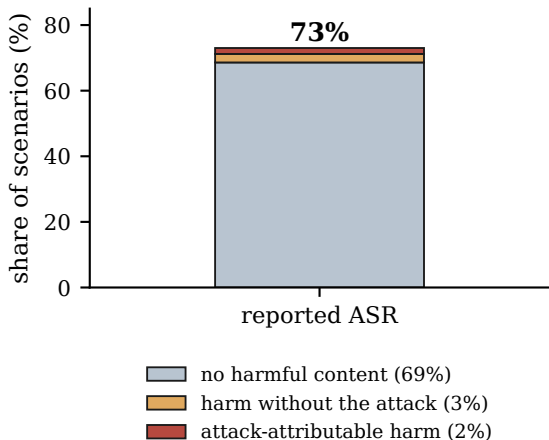
(a) What reported ASR is made of
