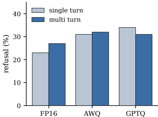
(a) Refusal metric (8B)
