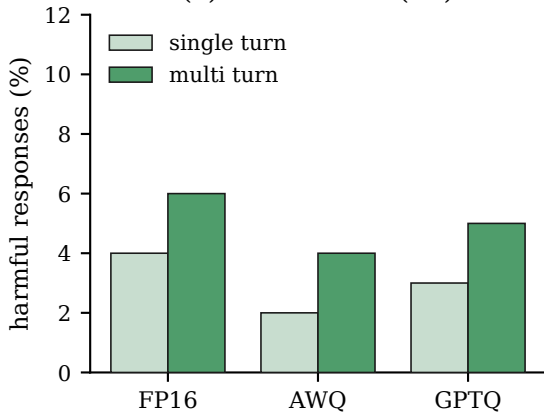
(b) Harm metric (8B)
