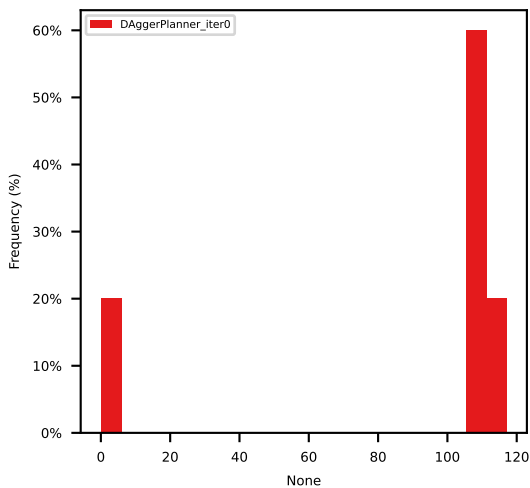
p90_ego_expert_l2_error_with_yaw
