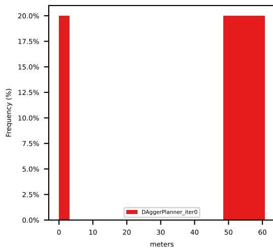
avg_ego_expert_L2_error
