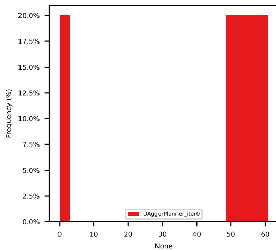
avg_ego_expert_l2_error_with_yaw
