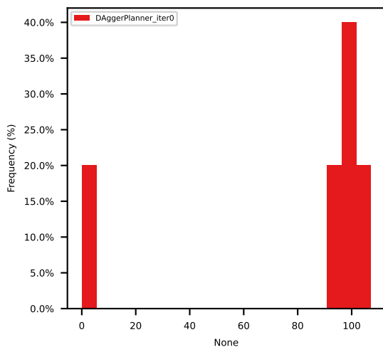
p90_ego_expert_l2_error_with_yaw
