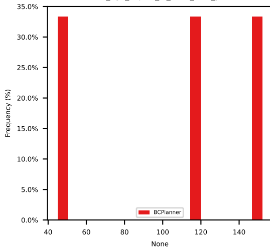
p90_ego_expert_l2_error_with_yaw
