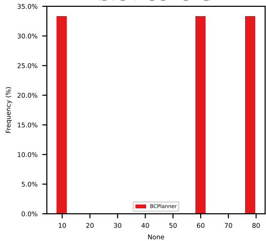
avg_ego_expert_l2_error_with_yaw
