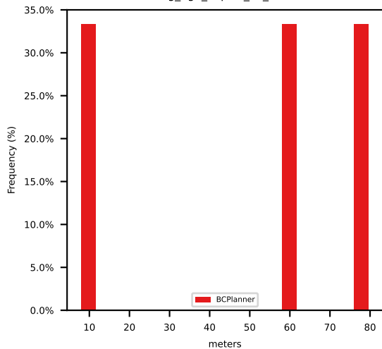
avg_ego_expert_L2_error
