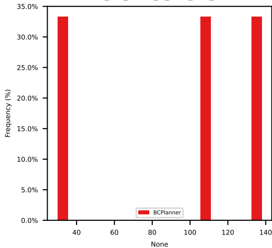
p90_ego_expert_l2_error_with_yaw
