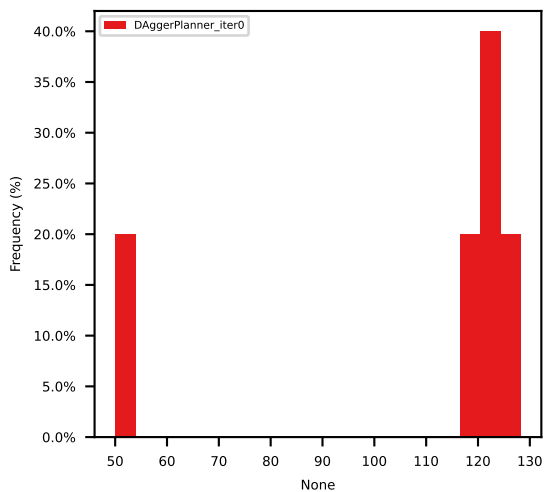
p90_ego_expert_l2_error_with_yaw
