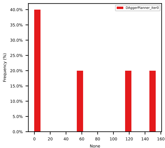
p90_ego_expert_l2_error_with_yaw
