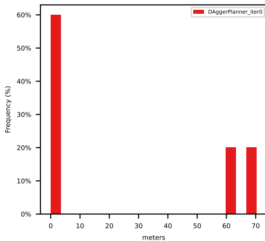
avg_ego_expert_L2_error
