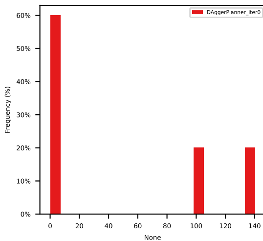
p90_ego_expert_l2_error_with_yaw
