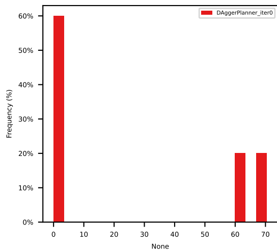
avg_ego_expert_l2_error_with_yaw
