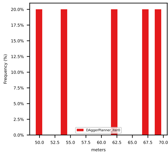
avg_ego_expert_L2_error
