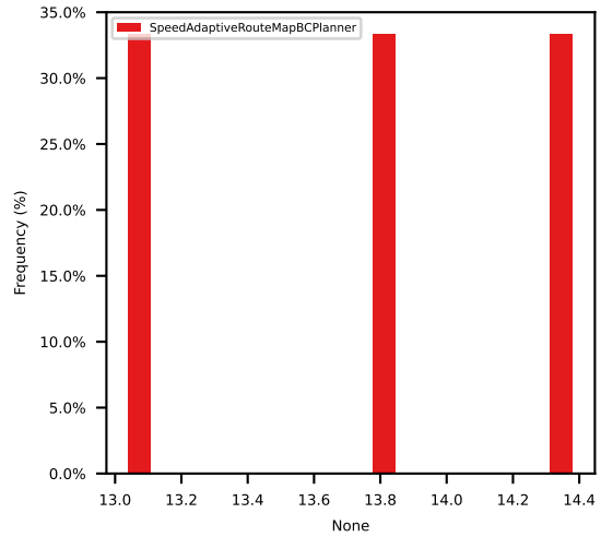
avg_ego_expert_l2_error_with_yaw
