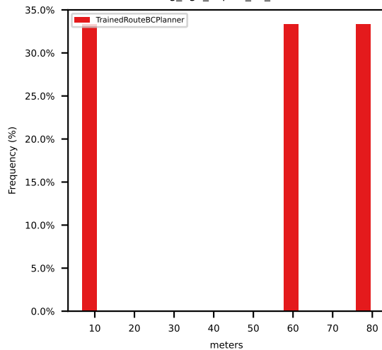
avg_ego_expert_L2_error
