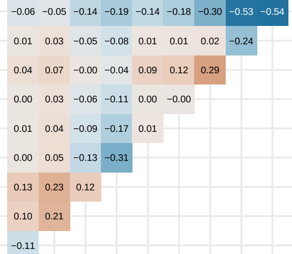
Mean Temperature
