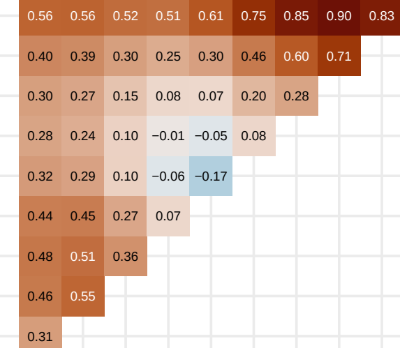
Relative Humidity
