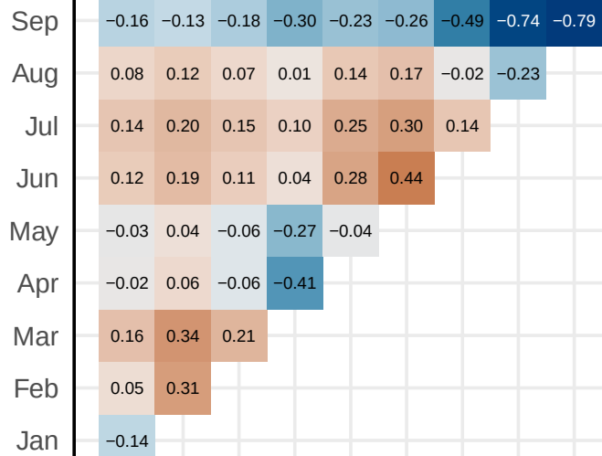
Maximum Temperature
