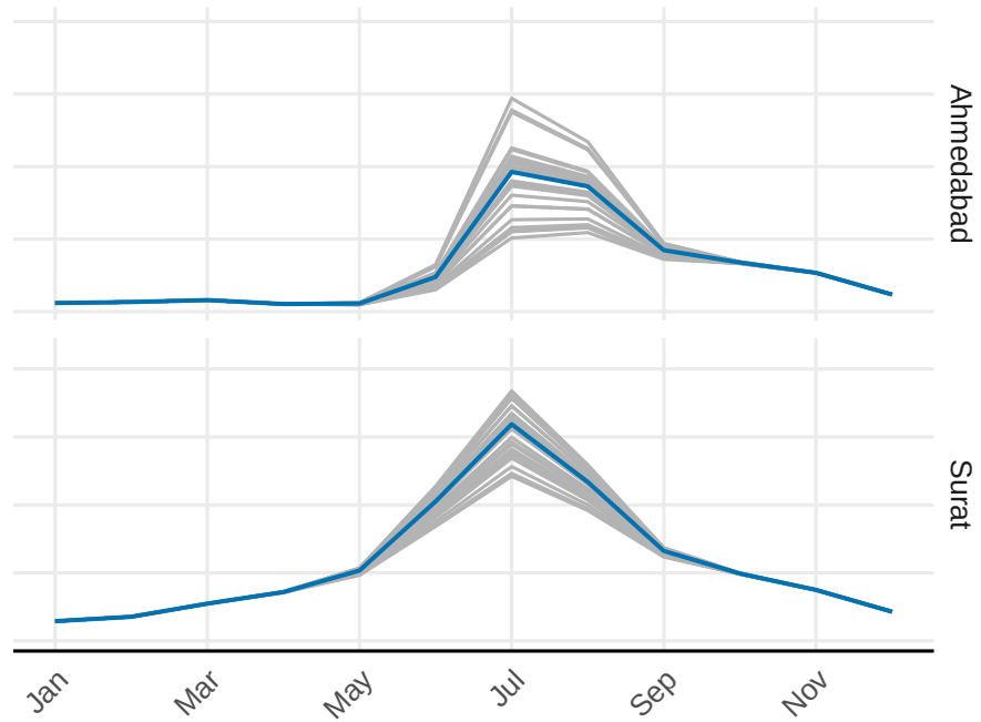
Relative Humidity
