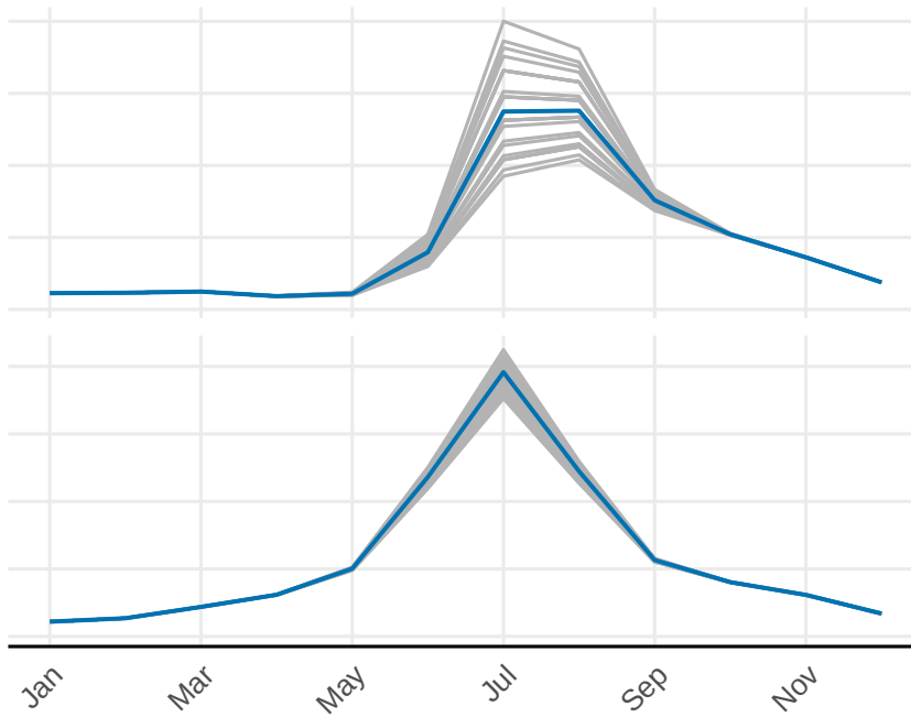
Maximum Temperature
