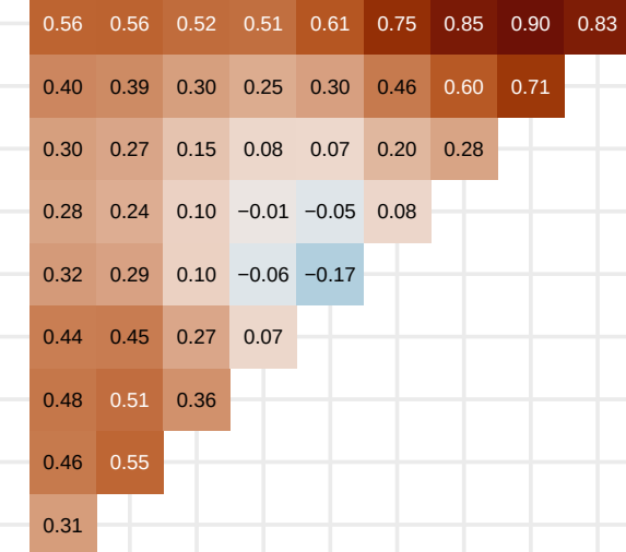
Relative Humidity
