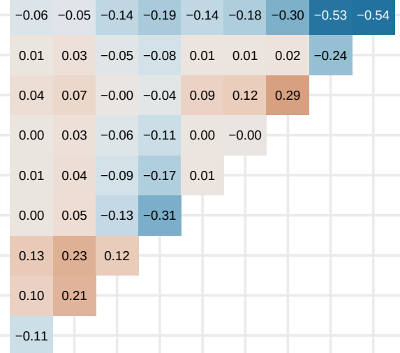
Mean Temperature
