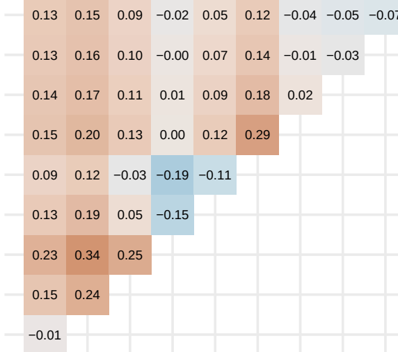
Minimum Temperature
