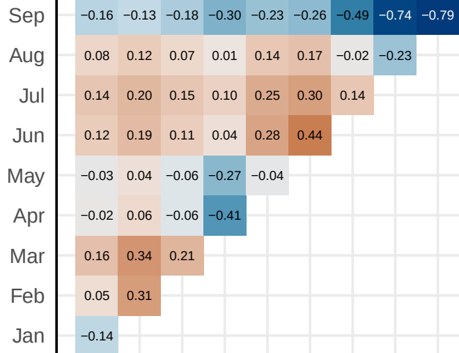
Maximum Temperature
