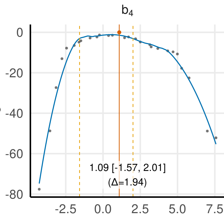
Relative log-likelihood
