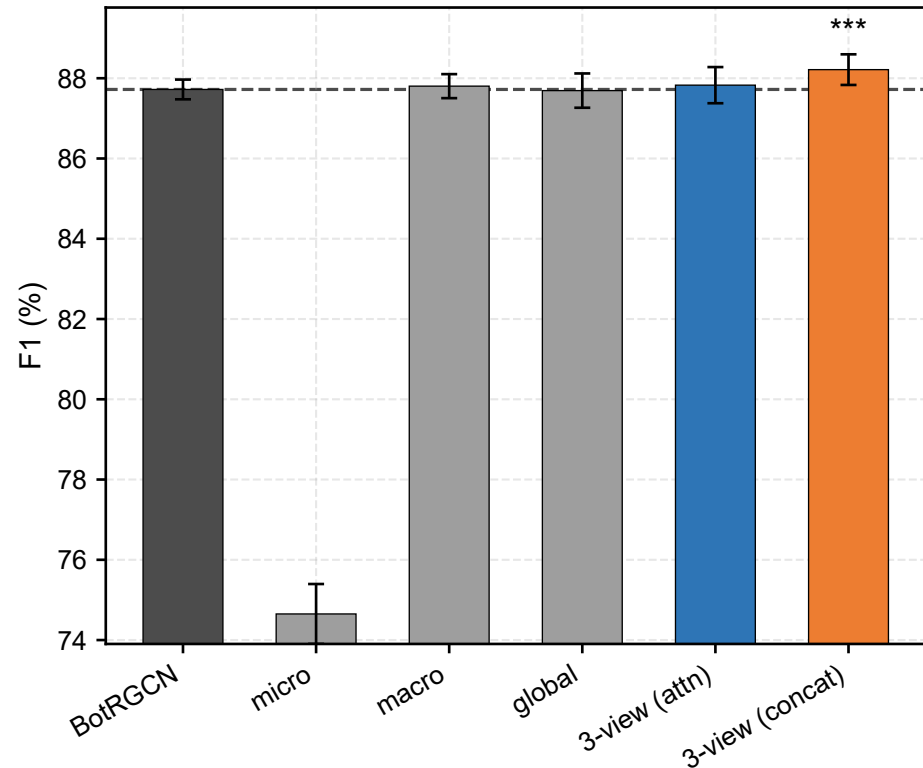
Twibot-20 Ablation (F1)
